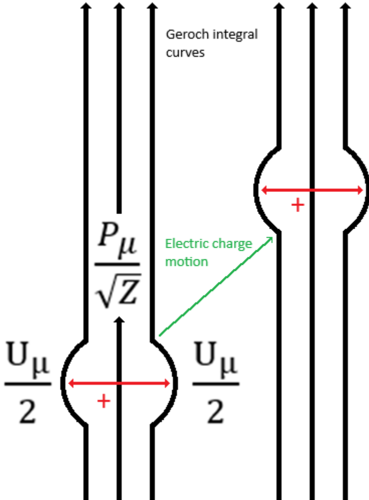
Fig. 2. – An over simplified charge in x-spacial horizontal and local Geroch-time axes \frac{P_{\mu}}{\sqrt{|Z|}}
